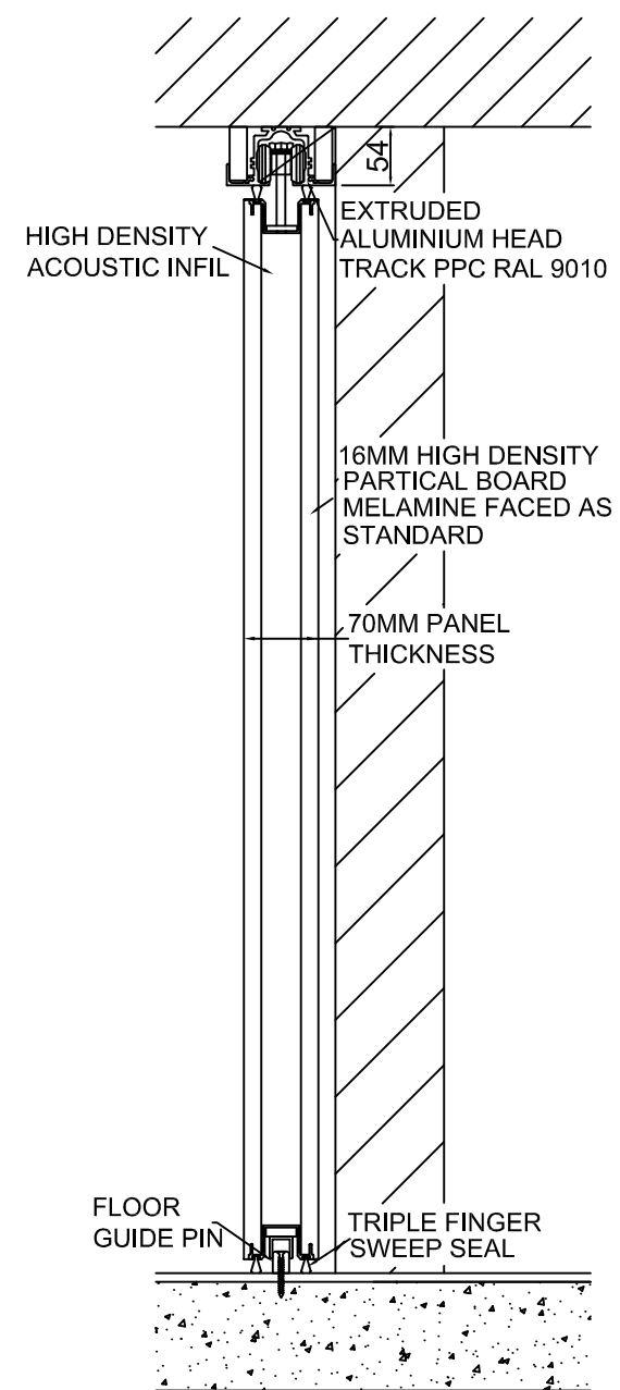
VERTICAL SECTION
